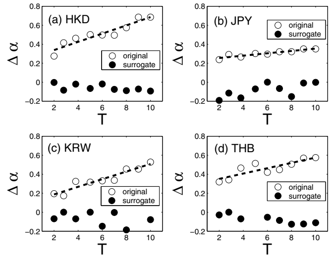
Fig. 5. The multifractality of time series from which returns above a threshold T\sigma have been deleted and interpolated. The panels refer to Hong-Kong (a), Japan (b), Korea (c), and Thailand (d). The open and fill circles indicate the original and surrogate time series.
