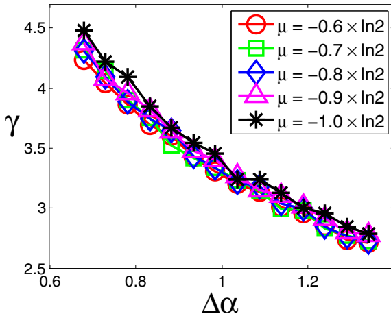
Fig. 4. (Color online) The relationship between the degree of multifractality and the tail exponent of power law distribution. We generate 100 multifractal noise data sets with 2^{17} data points with respect to \mu = \{-0.6 \times \ln 2, -0.7 \times \ln 2, -0.8 \times \ln 2, -0.9 \times \ln 2, -1 \times \ln 2\} and various \sigma values in the ranges from 0.2 to 0.4 and calculate the exponent of power-law distribution function. The circles (red), squares (green), diamonds (blue), triangles (pink), and stars (black) correspond to the multifractal noise data created with \mu = \{-0.6 \times \ln 2, -0.7 \times \ln 2, -0.8 \times \ln 2, -0.9 \times \ln 2, -1 \times \ln 2\} , respectively.
