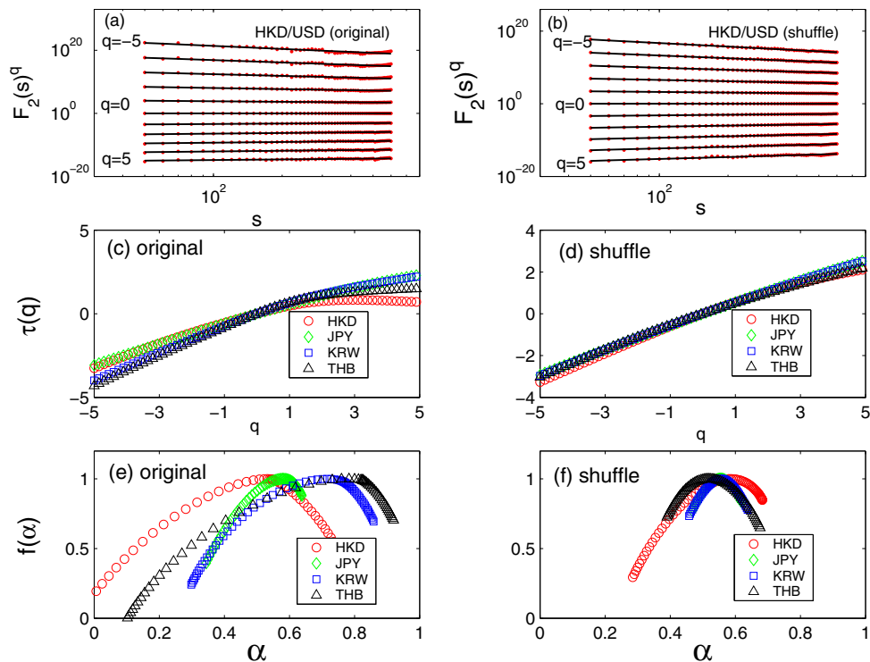
Fig. 2. (Color online) Panels (a) and (b) show the scaling function F_q(s)^q for various moments q of the Hong-Kong FX market, for the original (Fig. 1b) and surrogate (shuffled) time series respectively. Panels (c) and (d) show the multifractal scaling functions \tau(q) of the return and surrogate time series for all four foreign exchange markets. Panels (e) and (f) show the fractal dimension f(\alpha) obtained by a Legendre transformation of (c) and (d) respectively. Red circles refer to Hong Kong (HKD), green diamonds to Japan (JPY), blue squares to Korea (KRW), and black triangles to Thailand (THB).
