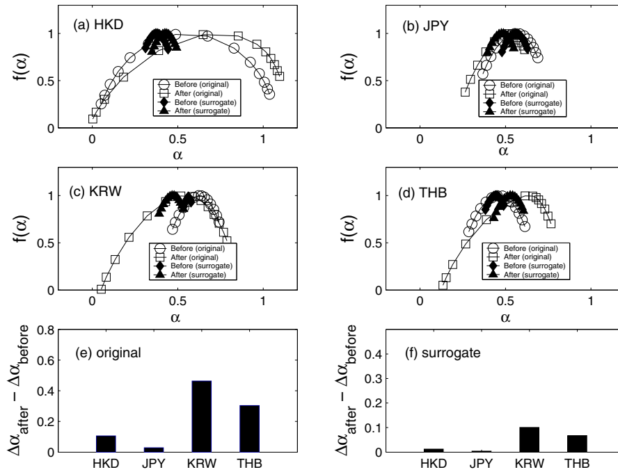
Fig. 3. The multifractality spectrum f(\alpha) , before (circles) and after (squares) the Asian currency crisis. The four panels refer to Hong Kong (a), Japan (b), Korea (c), and Thailand (d). Panel (e) and (f) plots the difference in the range of multifractality \Delta\alpha for the original and surrogate data.
