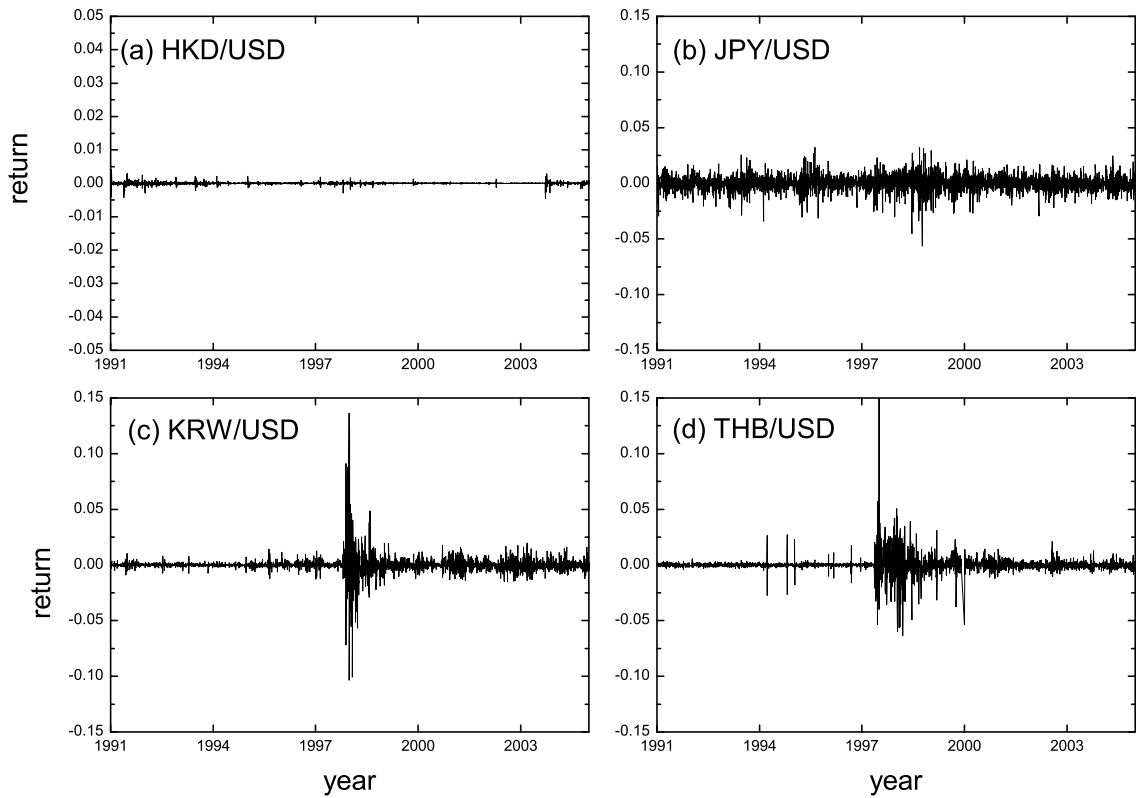
Fig. 1. Returns x(i) of four Asian foreign exchange markets: Hong-Kong (a), Japan (b), Korea (c), and Thailand (d).
