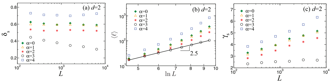
FIG. 6. (Color online) Successive slopes for d = 2 of (a) \delta_s obtained from \ln\langle \ell \rangle vs \ln L [of Fig. 5(b)], (b) \langle \ell \rangle as a function of \ln L in a double logarithmic plot, and (c) \gamma_s obtained from \ln\langle \ell \rangle vs \ln \ln L taken from (b). The total length \Lambda of the added long-range connections is limited to N = L^2 . Note that in (a) for \alpha = d + 1 = 3 , \delta_s decreases with L , while for other values of \alpha , \delta_s is roughly constant. In (c) for \alpha = d + 1 = 3 , \gamma_s keeps roughly constant and for other values of \alpha , \gamma_s increases with L . This suggests that for \alpha = 3 the relation between \langle \ell \rangle and L is a function that increases less than a power law and more likely that \langle \ell \rangle increases logarithmically with L .
