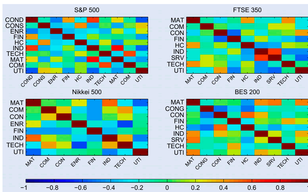
Figure 7. The correlation of influences from two sectors to the same stocks, i.e. \rho(d^{S_i}, d^{S_j}) , where d^{S_i} represents the vector variable of influence from sector i to all stocks. We represent the correlation using a heat map of closeness between sectors in different markets, using a colour code to represent the strength of the correlation, ranging from blue for full anti correlation, to red, for complete correlation. We observe that for the S&P 500 data, the pairs of industrials sector and consumer discretionary sector, materials sector and industrials sector and the communications sector and the technology sector are very close to each other, in terms of their influence, and an anti-correlation between the utilities sector and the consumer discretionary sector. For the case of the other three investigated markets—the UK FTSE 350 index, the Japanese Nikkei 500 index and the India BES 200 index—we find that all show high correlation between materials sector and industrials sector.
