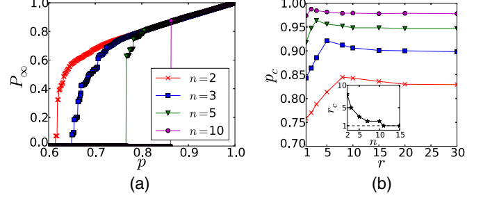
FIG. 6. (Color online) (a) Simulations of P_\infty , the fractional size of the giant component as a function of the fraction of surviving nodes p for n fully interdependent ( q = 1 ) spatial networks of size N = 100 \times 100 in a tree formation with r = 2 are shown. As the number of networks increases the transition becomes first-order (here at n = 5 ). (b) The percolation threshold p_c is plotted as a function of r (number of lattice units) for lattices with N = 250 \times 250 with symbols as defined in Fig. 6(a). The change from a second-order to a first-order transition occurs at r_c , when p_c reaches a maximum. The inset shows how this critical value, r_c , varies with the number of networks n . The critical dependency length can reach as low as r_c = 1 if there is a sufficient number of interdependent networks (here n = 11 ). Note that already at r = 30 the p_c becomes very close to the theory of Eqs. (3) and (4) for r = \infty . In this case since a fraction 1 - p was removed from all networks, we must take p_c^{1/n} in order to get results that agree with Eqs. (3) and (6) and Fig. 5(a). The lines in this figure are a guide to the eye.
