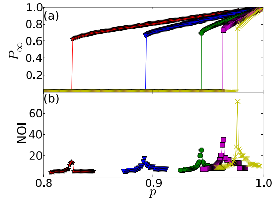
FIG. 4. (Color online) (a) Theory (lines) and simulations (symbols) of the size of the giant component, P_\infty(x) , as a function of the fraction of surviving nodes p , for networks of interdependent lattices of size N = 250 \times 250 with treelike structure are shown. These results are again for a network of networks in a line yet the results are the same for any other tree formation. Results are shown for n = 2 (red stars), n = 3 (blue triangles), n = 5 (green circles), n = 7 (purple squares), and n = 10 (yellow-green x's). As shown, all of the transitions are first order and the simulations fit well with the theory. Further, increasing the number of networks is seen to quickly increase p_c , indicating that the system becomes more vulnerable as n increases. (b) Here we observe that the number of iterations (NOI) it takes for the system to arrive at steady-state diverges at the critical threshold p_c . The number of iterations at p_c increases both with the number of networks, n , and the size of the networks, N [51].
