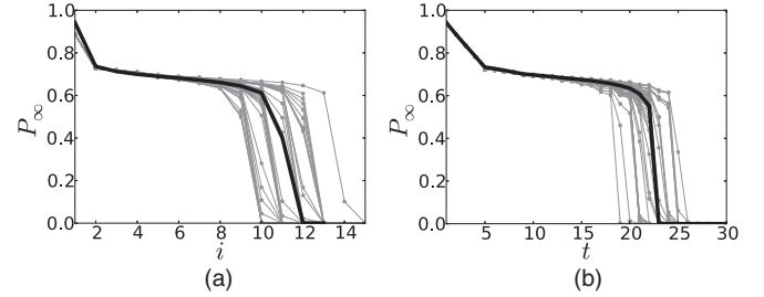
FIG. 3. Theory for P_\infty(x) , the size of the giant component, after a number of iterations is shown as the thick black curve and 40 simulated realizations on lattices of size N = 500 \times 500 are shown as the lighter curves at p = 0.942 < p_c = 0.944 . (a) P_\infty as a function of the number of iterations, i , is shown to fit well with the theory of Eq. (1). These results are for five networks in a line, yet for this method the shape of the tree has no effect on the number of iterations. (b) P_\infty as a function of t iterations according to the method in Gao et al. [21] for five networks in a line fits well with the theory.
