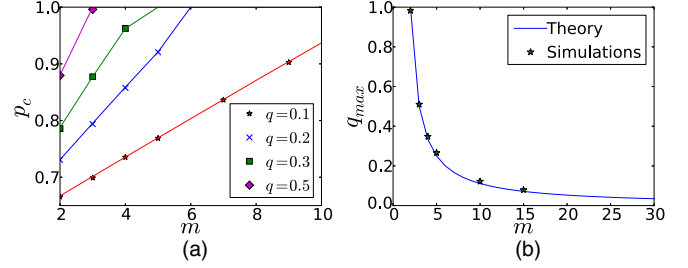
FIG. 8. (Color online) (a) The critical threshold p_c for an RR network of spatial networks is plotted as a function of m , the number of dependencies each network has for several fractions of interdependent nodes q . The lines represent the theory according to Eq. (10) and the symbols represent simulations. It is worth noting that once the number of dependencies reaches a certain value, p_c \rightarrow 1 for a given q value. This q value represents q_{\max} , the maximum dependency the system can sustain. (b) The maximum coupling fraction between networks, q_{\max} , above which p_c \rightarrow 1 is plotted as a function of m . As seen, q_{\max} decreases rapidly with m , indicating that as each network has more dependencies less coupling is required for the network to fail after even the smallest attack. Simulations (symbols) on lattices of size N = 250 \times 250 are shown to fit well with the theory of Eqs. (13) and (14) (lines).
