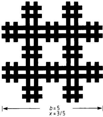
Figure 1. Example of a fractal embedded in a square lattice with b=5 and x=3/5 . Two stages of the fractal are shown.
