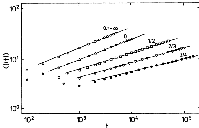
FIG. 2. Plot of \langle l(t) \rangle vs t for various \alpha .
