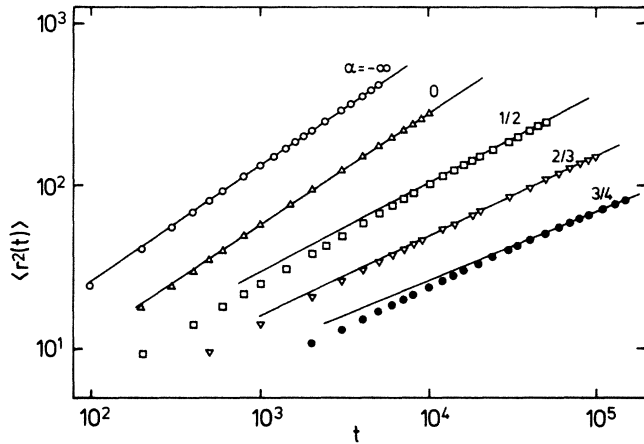
FIG. 1. Plot of \langle r^2(t) \rangle vs t for various \alpha . For our calculations, we generated clusters up to 150 shells (typically 10000 sites) using the Leath algorithm (Ref. 12). To determine \langle r^2(t) \rangle , we used the exact enumeration for the "blind ants," Eqs. (9)–(11). For each value of \alpha we averaged over 400 configurations each.
