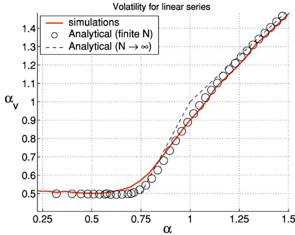
FIG. 1. (Color online) Magnitude series scaling exponent \alpha_v vs the two-point correlation exponent \alpha for linear sequences u_i . The solid line represents results for synthesized sequences of length 2^{15} , averaged over 15 configurations, for u_i^2 and |u_i| (these two coincide). The circles represent the analytical reconstruction taking into account corrections due to finite size effects and nonstationarity. Analytical results for N \rightarrow \infty are given by the dashed line.
