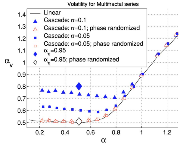
FIG. 2. (Color online) The magnitude series exponent \alpha_v vs the two-point correlation exponent \alpha for multifractal series. The full triangles and squares represent sequences generated by the log-normal random cascade algorithm with \sigma=0.1 (triangles) and \sigma=0.05 (squares); the multifractal spectrum of these examples is known analytically indicating that as \sigma increases the nonlinearity strengthens. The respective linear (phase randomized) surrogate data sequences are represented by empty symbols. The solid line indicates simulation results for linear sequences as derived in [17], explained in Sec. III, and shown in Fig. 1. The full diamond represents the scaling exponent of our multifractal model's sequences u_i = \epsilon_i \eta_i with \alpha_\eta = 0.95 , while the empty diamond represents the respective scaling exponent of the surrogate data. All sequences are of length 2^{14} elements, and results were averaged over 15 configurations. Error bars are smaller than symbol size.
