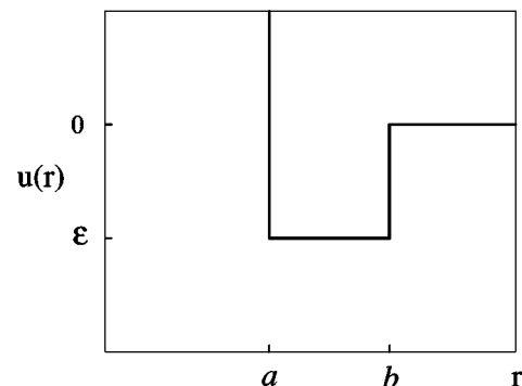
FIG. 1. Square-well potential. The ratio of the attractive distance b to the hard-core repulsive distance a is b/a = \sqrt{3} . The depth of the square-well \epsilon = -1.0 is the interaction energy per pair of particles.
