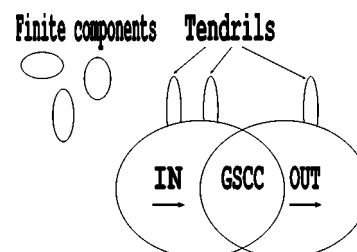
FIG. 1. Structure of a general directed graph.
